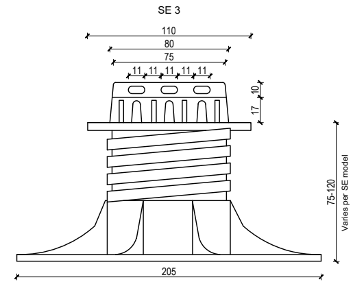
ELEVATION (JOIST LEVELLING HEAD)
