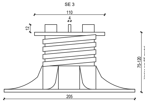
ELEVATION (TILE LEVELLING HEAD)
