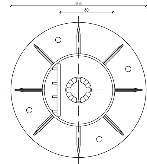
PLAN (JOIST LEVELLING HEAD)
