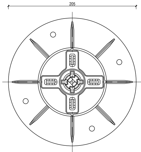
PLAN (TILE LEVELLING HEAD)
